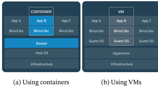
Figure 5.1. Comparison between containers and VMs (from docker.com )
