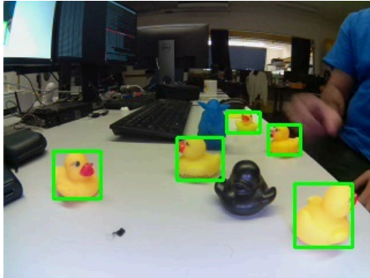
Figure 4.1. Sample Yellow Color Detector
